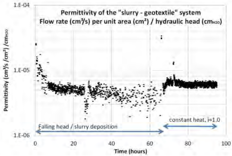
Figure 9 Permittivity versus time
