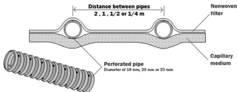
Figure 1 Multi-Linear drainage geocomposite
