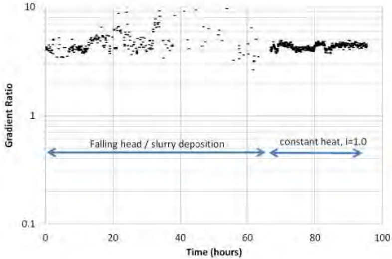
Figure 10 Gradient ratio versus time
