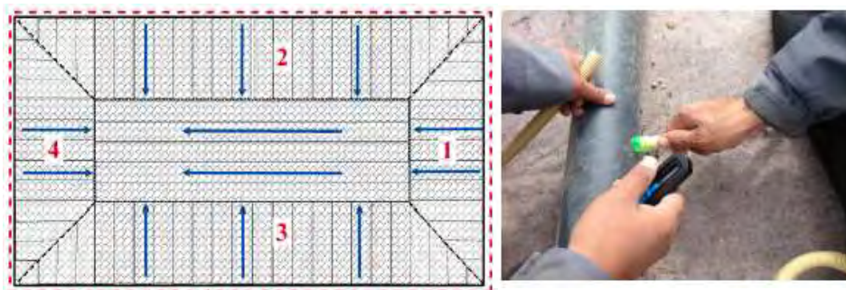
Figure 12: orientation of the MLDG and connection using connectors (photo courtesy Afitex-Textel)
